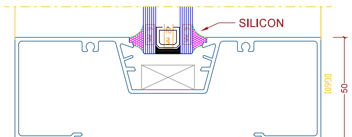
24mm GLASS
