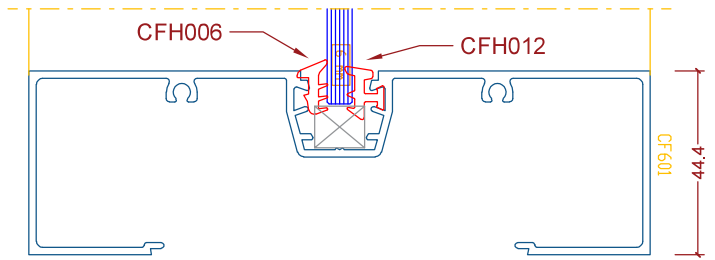
8mm GLASS
