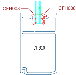
6mm GLASS
