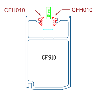
10mm GLASS
