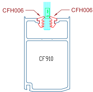
6mm GLASS
