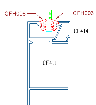
6mm GLASS
