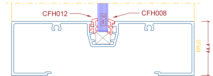
8mm GLASS
