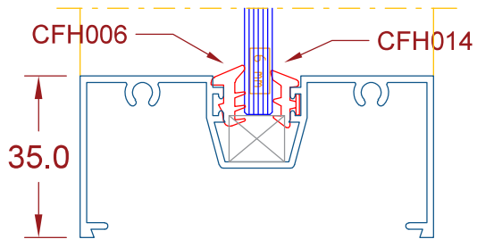
6mm GLASS
